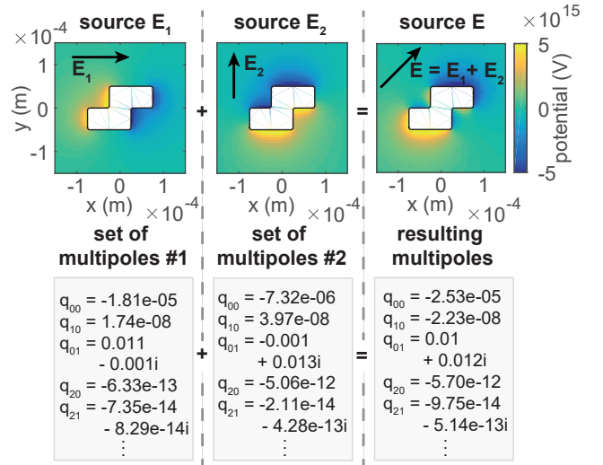
Fig. 5. Illustration of the superposition principle utilization.
