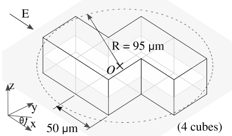
Fig. 3. Dimensions of the Tetrish-shaped micro-object used in the example and validation simulations.
